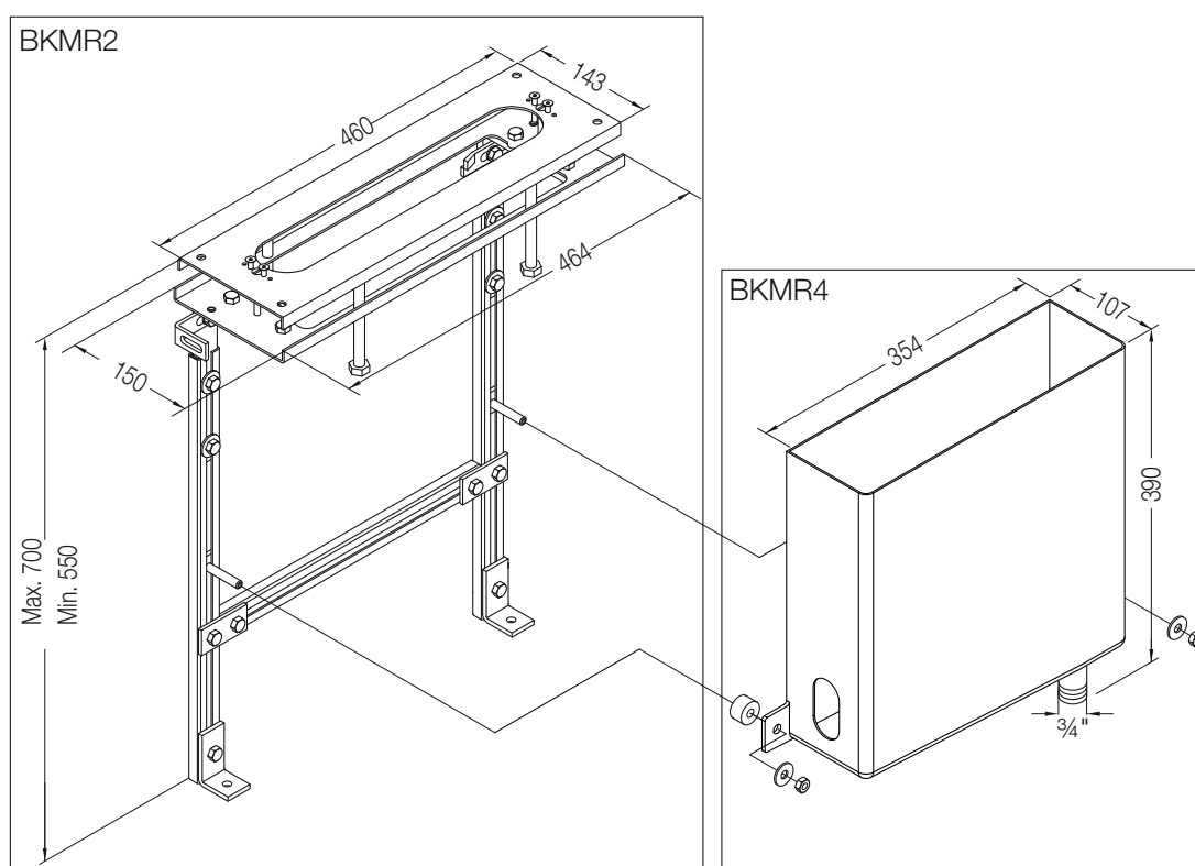
Montageramme og boks BK 3/4/6/8/10/11/12/13/14/15/16
