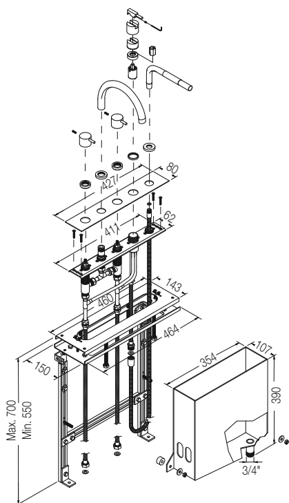
Komplet system (BK system)
